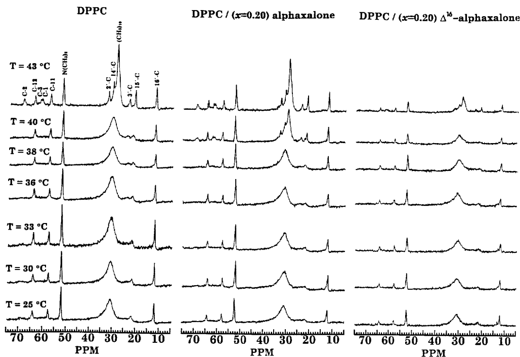
Fig. 7. The hydrophobic, glycerol and backbone regions of ^{13}\text{C} -MAS spectra of bilayer preparations of DPPC, DPPC + alpha-xalalone, and DPPC + \Delta^{16} -alpha-xalalone in the temperature range of 25–43°C.
