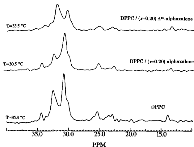
Fig. 5. The hydrophobic region of ^{13}\text{C} -CP/MAS spectra of bilayer preparations of DPPC at 35.3°C, DPPC + alphaxalone at 30.5°C, and DPPC + \Delta^{16} -alphaxalone at 33.5°C.
