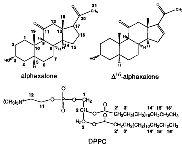
Fig. 1. Chemical structures of alphaxalone, \Delta^{16} -alphaxalone, and DPPC.
