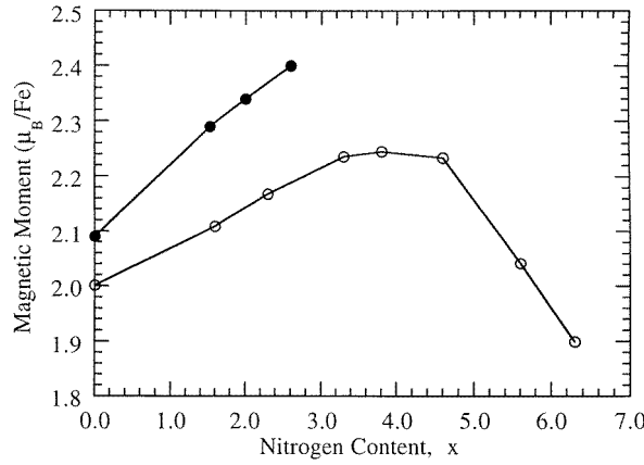
Figure 5. The average magnetic moment per Fe atom (in \mu_B ) versus the N content x for Y_2Fe_{17}N_x ( 0 \leq x \leq 6.3 ): open circles—nitrided with NH_3 gas (this work), closed circles—nitrided with N_2 gas [17].
