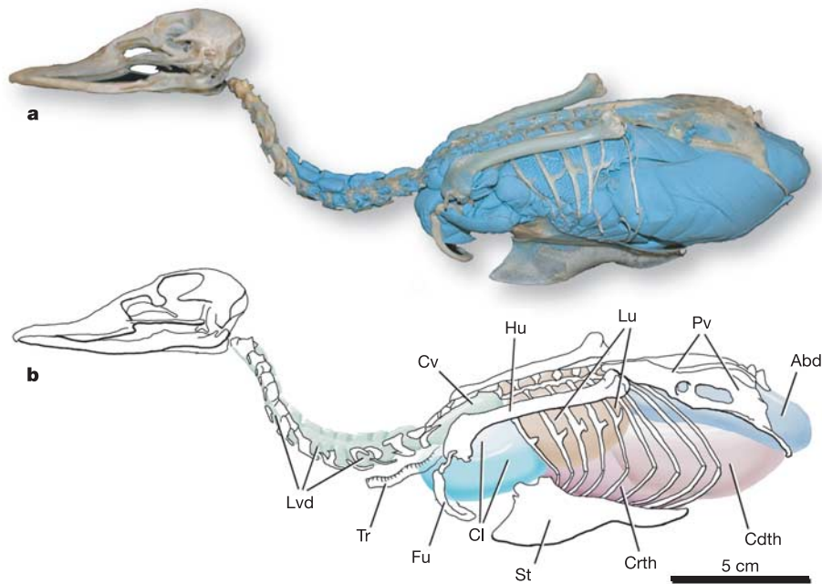
Figure 1 | Pulmonary air-sac system in a bird. a , Latex injection (blue) of the pulmonary system in a duck ( Anas crecca ), highlighting the extent of air sacs throughout the body. b , Main components of the avian flow-through system (ribs have been illustrated in their proper anatomical positions).
