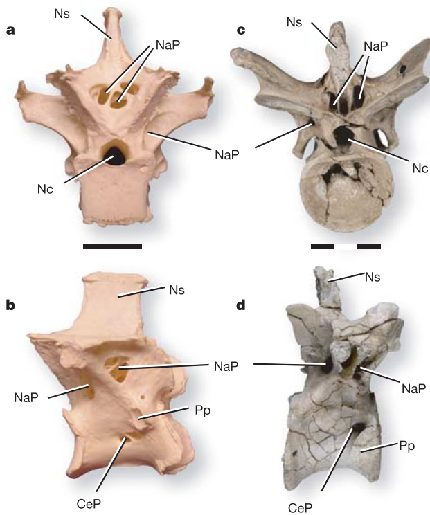
Figure 3 | Vertebral pneumaticity in avian and non-avian theropods. Comparisons between a bird ( a, b ) and theropod dinosaur ( c, d ) in caudal ( a, c ) and right lateral ( b, d ) views, illustrating the topological similarity of pneumatic features. a, b , Cranial thoracic vertebra of a sarus crane ( Grus antigone , SBU AV104063). c, d , Mid-cervical ( c ) and cervicothoracic ( d ) vertebra of an abelisauroid theropod ( Majungatholus atopus , UA 8678). Scale bar, 1 cm ( a, b ) and 3 cm in ( c, d ). CeP, central pneumatic foramen; NaP, neural arch pneumatic foramen; Nc, neural canal; Ns, neural spine; Pp, parapophysis.
